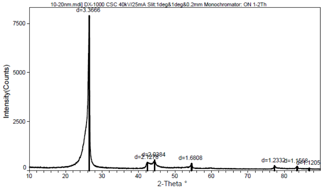
X-ray diffraction pattern
